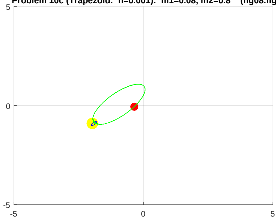
Celestial Mechanics: Two (2) Body Problem Problem 10c (Trapezoid: h=0.001 ): m_1=0.08 , m_2=0.8 (fig08.fig)
